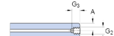
OH 3072 H Bearing 2D drawings and 3D CAD models
